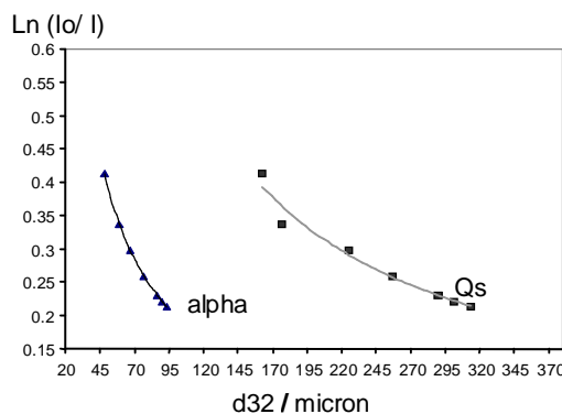
Fig. 11 A plot of d_{32} and \ln(I_o / I) at j = 0.005
