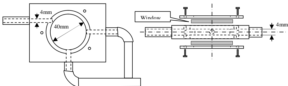
Fig. 5 Schematic diagram of the flow cell
