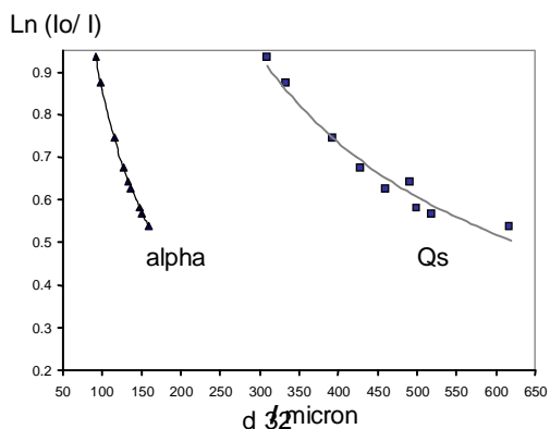
Fig. 8 A plot of d_{32} and \ln(I_o / I) at j = 0.02
