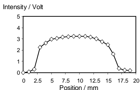
Fig. 6 Intensity profile of He-Ne laser beam
