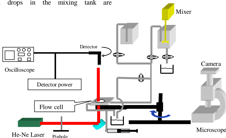
Fig. 4 The experimental setup
