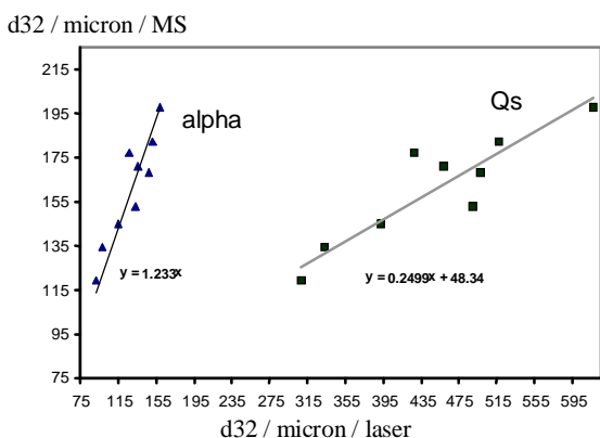
Fig. 13 Comparison of d32 between MS with laser (alpha & Q s ) at j = 0.02
