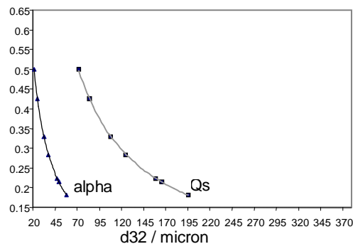
Fig. 12 A plot of d_{32} and \ln(I_o / I) at j = 0.0025
